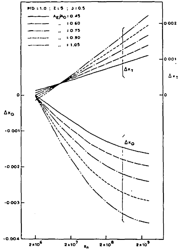
Figure 5. Influence of blade area ratio on Reynolds number effect on thrust and torque coefficients.
