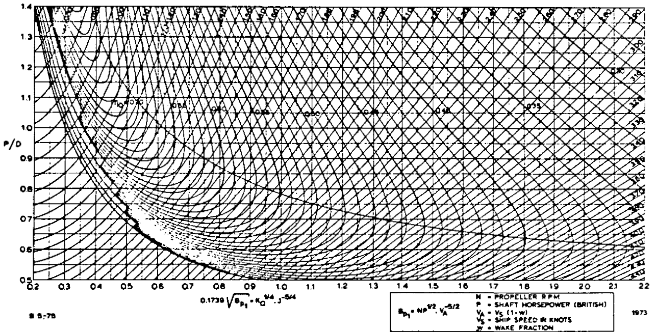
Figure 9. K_Q^{1/4} \cdot J^{-5/4} - J^{-1} diagram of B5-75 propeller according to polynomials given in Table 5 ( R_n = 2 \times 10^6 ) for determination of optimum diameter.
