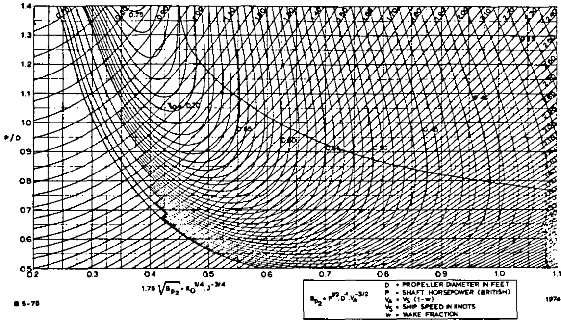
Figure 10. K_Q^{1/4} \cdot J^{-3/4} - J^{-1} diagram of B5-75 propeller according to polynomials given in Table 5 ( R_n = 2 \times 10^6 ) for determination of optimum diameter.
