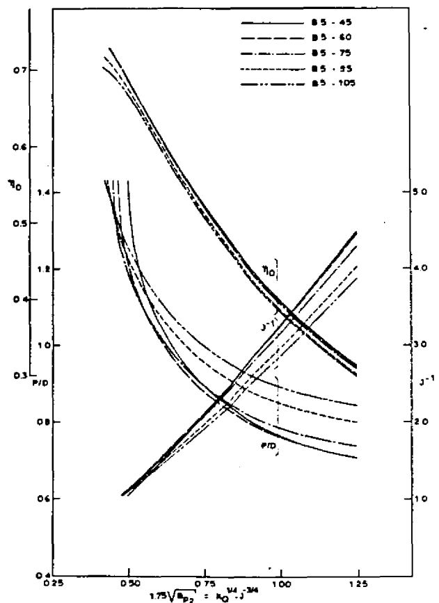
Figure 12. Values of pitch-diameter ratio and J^{-1} corresponding to optimum RPM (based on K_Q^{1/4} \cdot J^{-3/4} ).
