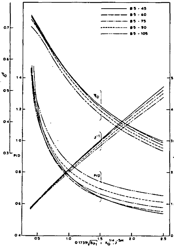
Figure 11. Values of pitch-diameter ratio and J^{-1} corresponding to optimum diameter (based on K_Q^{1/4} \cdot J^{-5/4} ).
